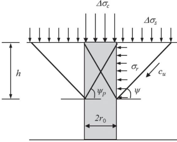
Figure 3. Failure mode of a single column [30]
