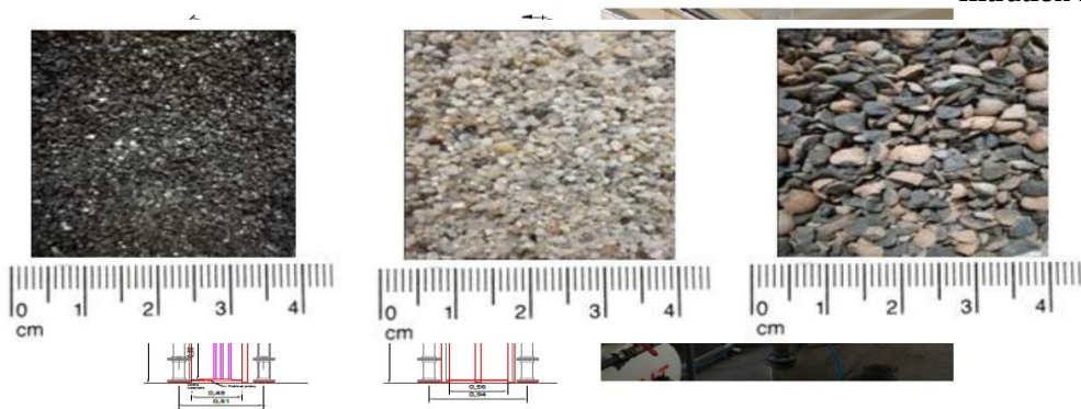
Figure 2. View of filtration media beds used in the pilot-scales of BAF
