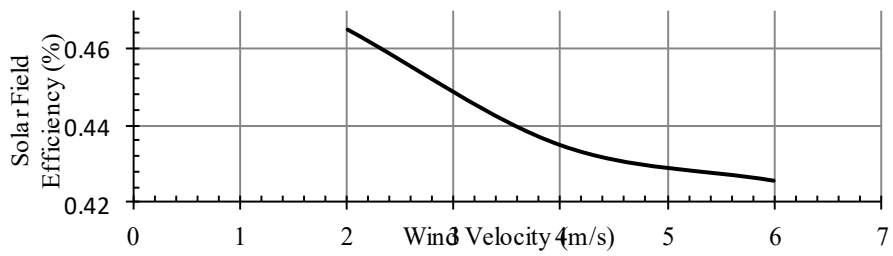
Figure 4.19: Effect of Wind Velocity on Solar Field Efficiency.
