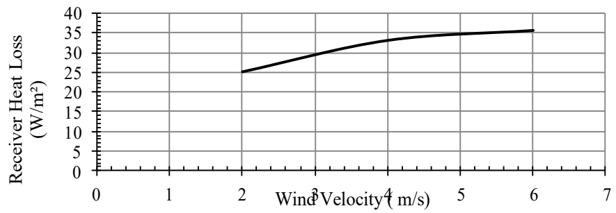
Figure 4.20: Effect of Wind Velocity on Receiver Heat losses.
