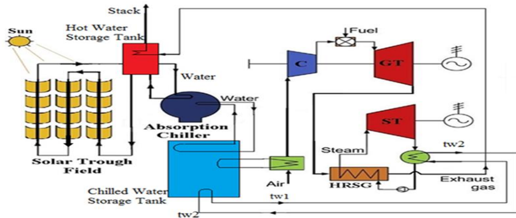
Figure 3.1: Schematic diagram of the proposed solar cooling system in Benghazi North power plant.
