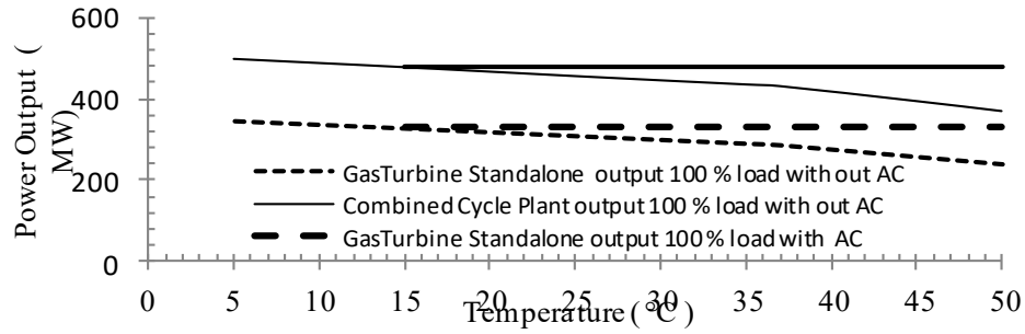
Figure 4.1: Effect Of Ambient Temperature On Benghazi North Power Plant Output.
