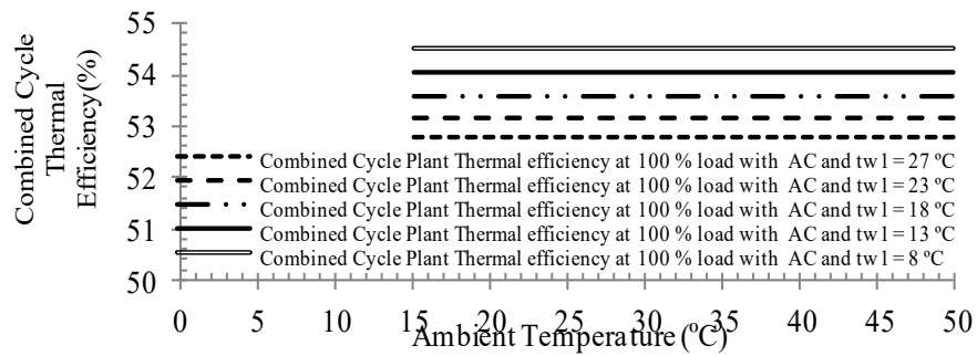
Figure 4.5: Effect of Condenser Inlet Cooling Water Variations on Benghazi North plant Thermal Efficiency with air cooling .
