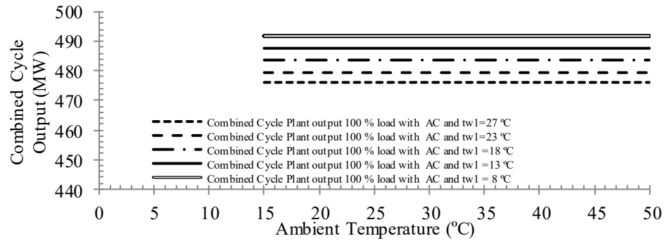
Figure 4.4: Effect of Condenser Inlet Cooling Water Variations on Benghazi North
