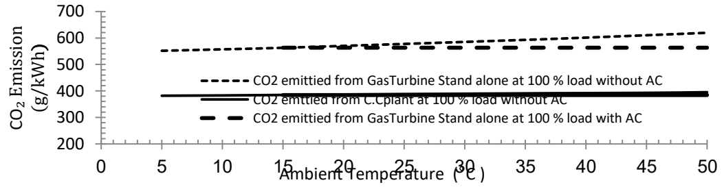
Figure 4.9: Effect Of Ambient Temperature On Benghazi North Power Plant CO 2 Emission.
