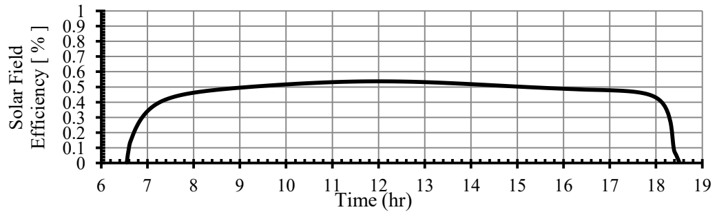
Figure 4.13 Solar Field Efficiency Variation during operation hours of august 16.
