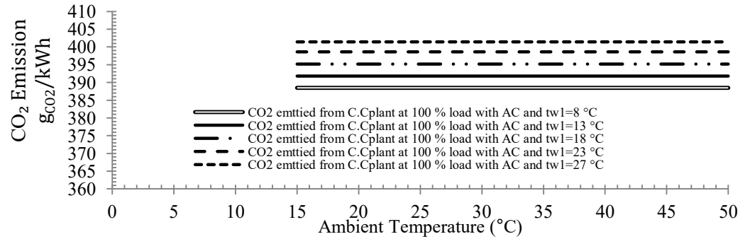
Figure 4.10: Effect of Condenser Inlet Cooling Water Variations on Benghazi North plant with Intake Air cooling CO 2 Emission.
