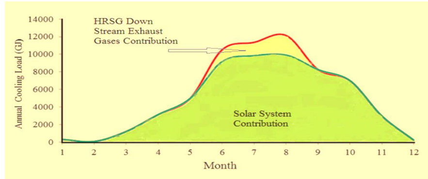
Figure 4. 23: Contribution of Solar System Integrated with HRSG Waste Heat Covering Annual Cooling Load of Benghazi North Power Plant Intake Air 4.1.Estimation of initial, operation and maintenance costs:
