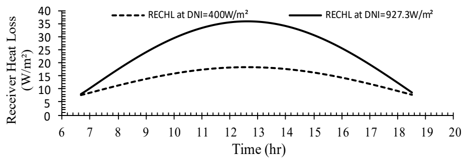
Figure4.15: Effect of Direct Normal Insolation on Receiver Heat Loss.
