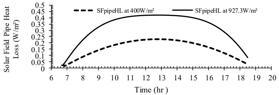
Figure 4.16: Effect of Direct Normal Insolation on Solar Field Pipe Heat Loss.
