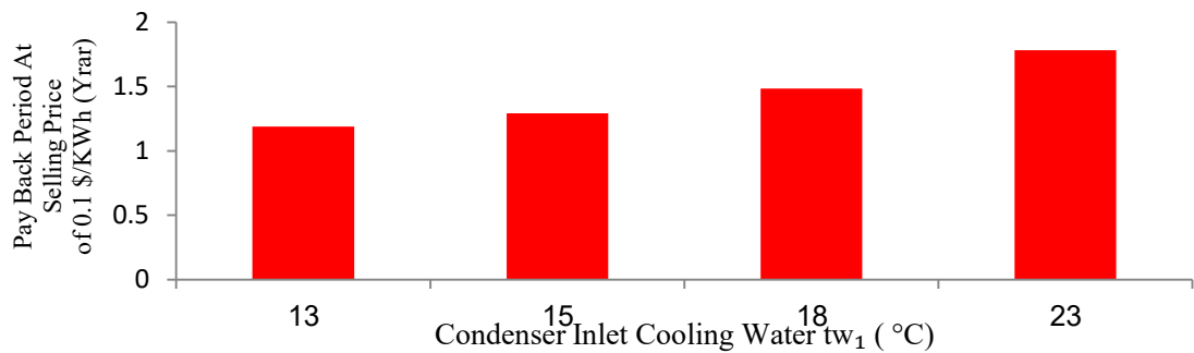
Figure 4.24: Effect of Condenser Inlet Cooling Water on Payback Period.
