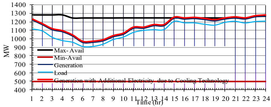
Figure 4.21: Libyan Eastern Network Daily Load Curve August 16.
