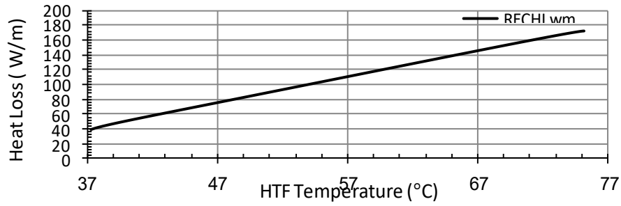
Figure 4.12. Receiver heat loss vs. bulk fluid temperature
