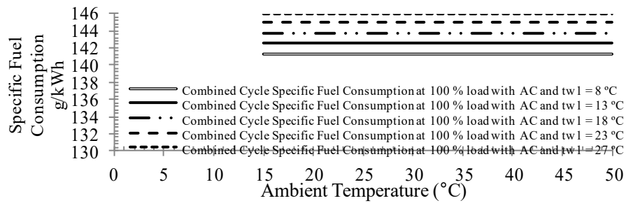
Figure 4.8 Effect of Condenser Inlet Cooling Water Variations on Benghazi North plant Specific Fuel Consumption with Intake Air Cooling .
