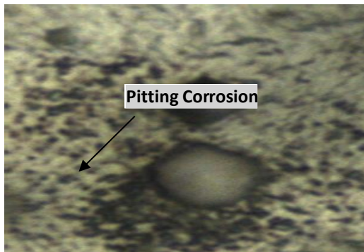
Fig. (3.5) SS 309L samples after 265 hrs. of Exposure in NaCl showing traces of pitting corrosion. 1000X.
